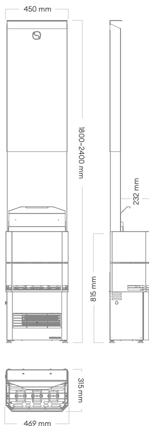
4,5/6 kW
