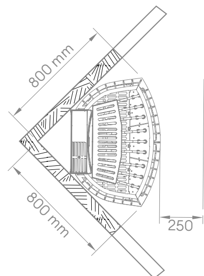
Nurka paigaldus
